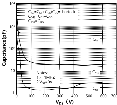
Figure 5. Capacitance Characteristics
